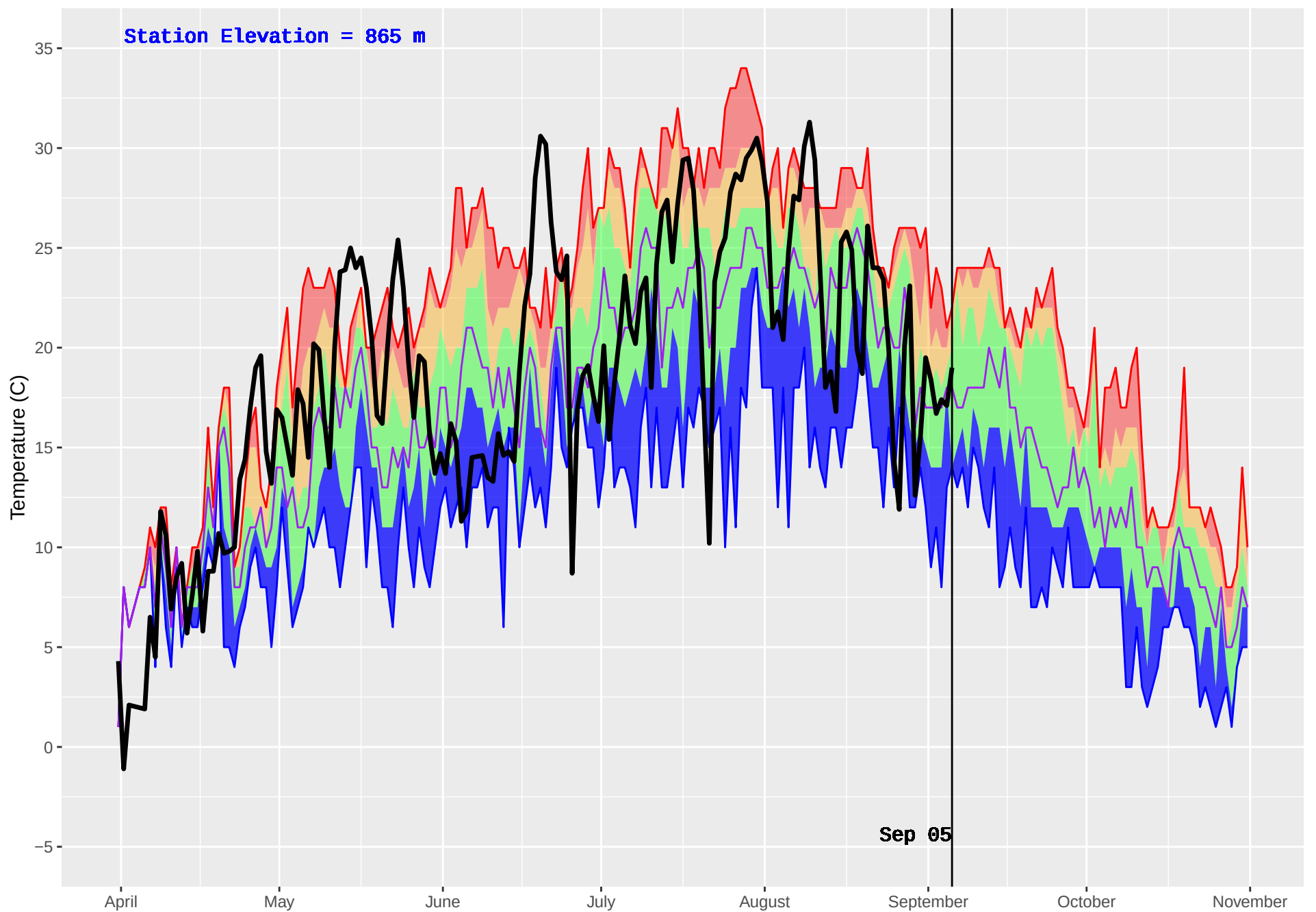
FIVE MILE (1029) : Historical (2008–2016) and Current (2018) Daily Temperature
