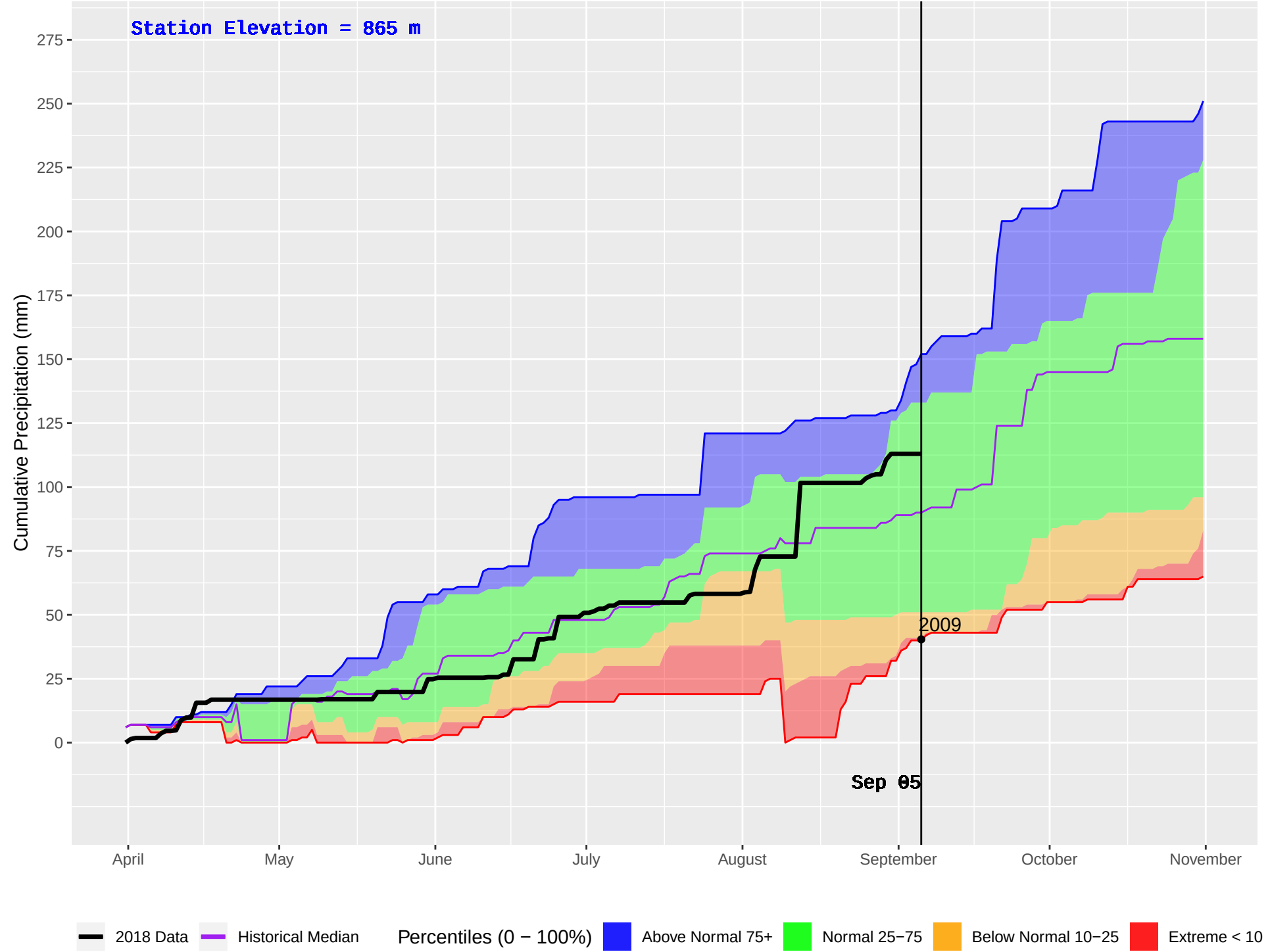
FIVE MILE (1029) : Historical (2008–2016) and Current (2018) Daily Cumulative Precipitation
