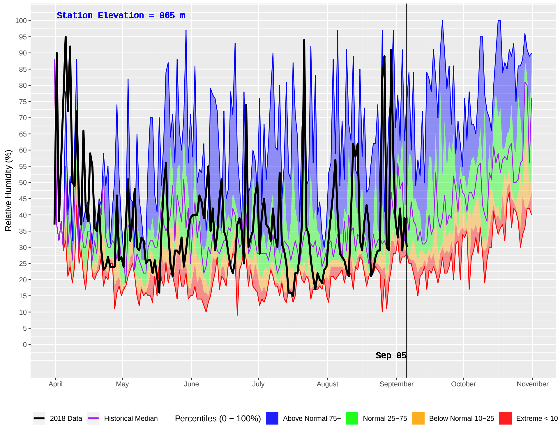
FIVE MILE (1029) : Historical (2008–2016) and Current (2018) Daily Relative Humidity
