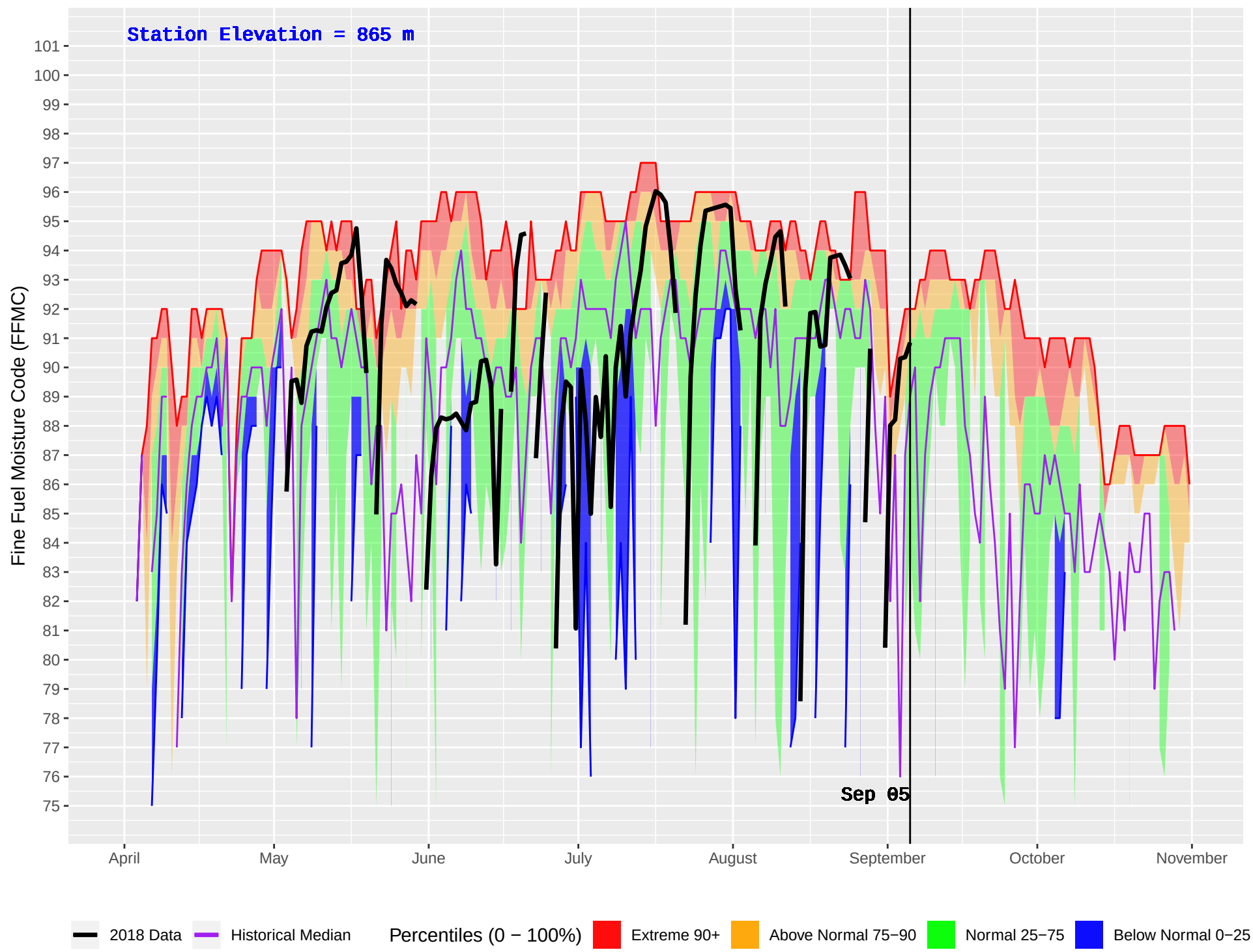
FIVE MILE (1029) : Historical (2008–2016) and Current (2018) Daily Fine Fuel Moisture Code (FFMC)
